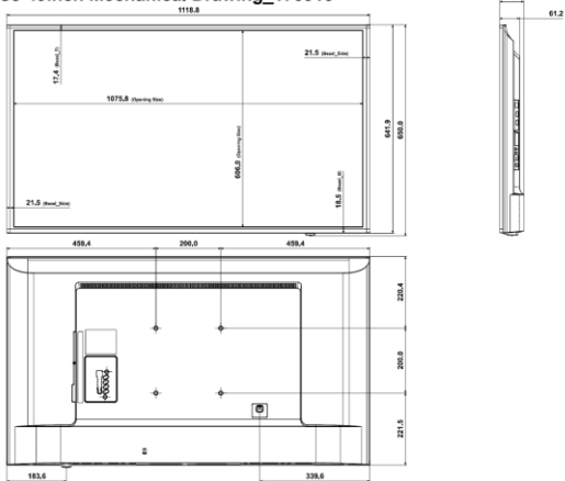
DBJ/DCJ 49inch Mechanical Drawing_170913
