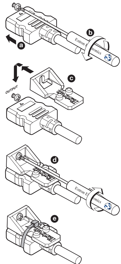
Figure 4. LockIt Bracket Installation Steps
