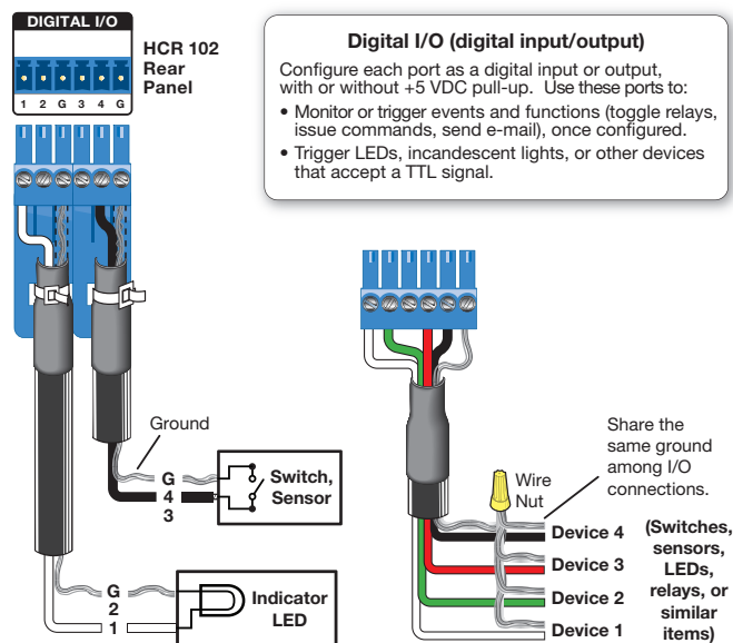
Figure 7. Digital I/O Port Wiring Examples
