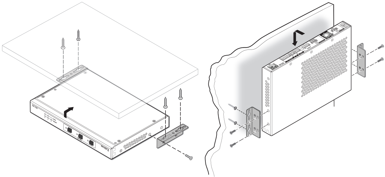
Figure 25. Mounting the Transmitter (Left) and the Receiver (Right)
