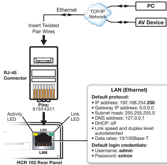
Figure 8. LAN Connector and LEDs
