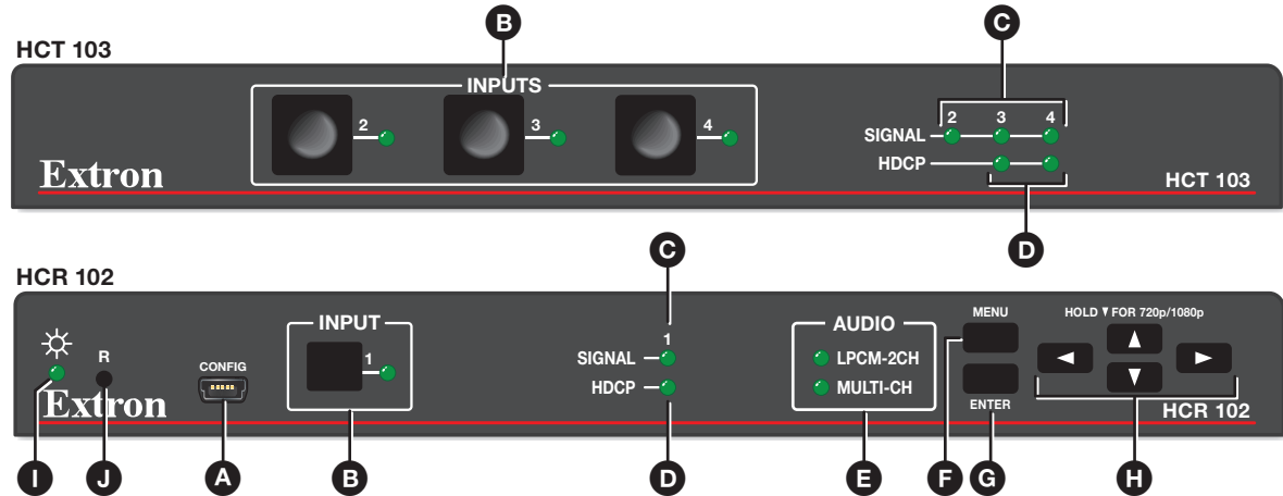
Figure 2. HCT 103 Front Panel (Top) HCR 102 Front Panel (Bottom)
