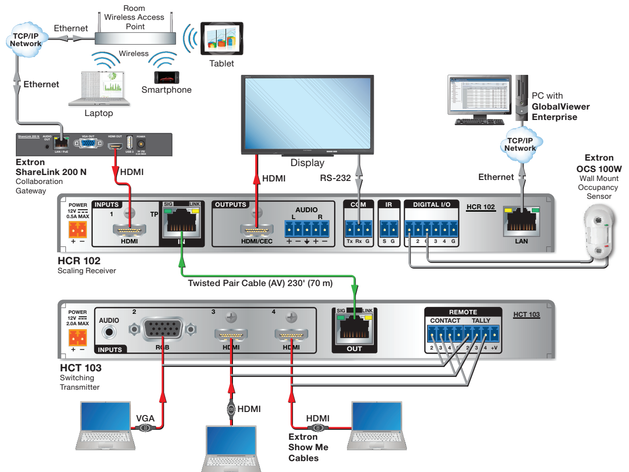
Figure 1. A Typical TeamWork HC 404 System Application
