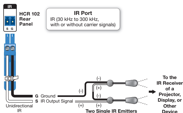
Figure 6. Wiring the IR Port
