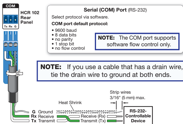
Figure 5. Wiring the COM Port for Serial Control
